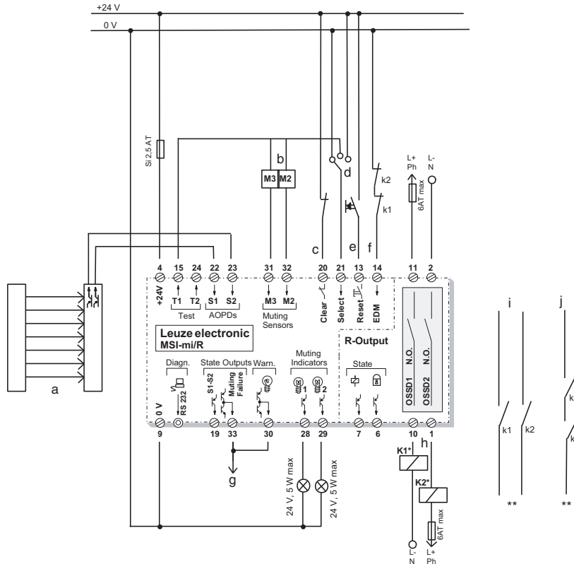
Connection example MSI-mi/R with one AOPD Type 4
