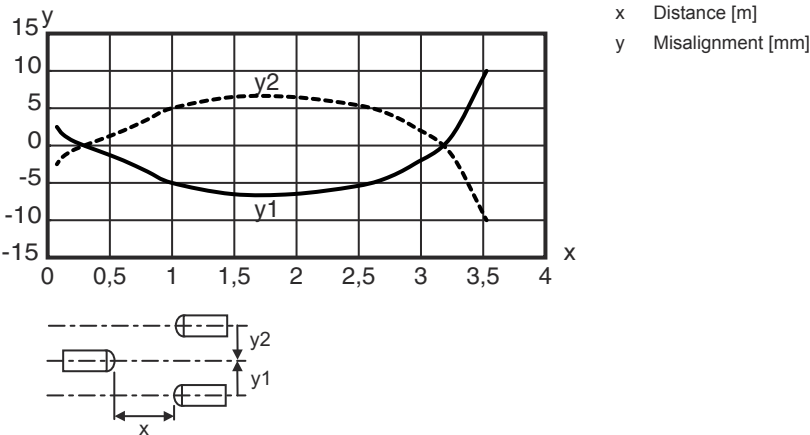
Typ. response behavior (TKS100x100)
