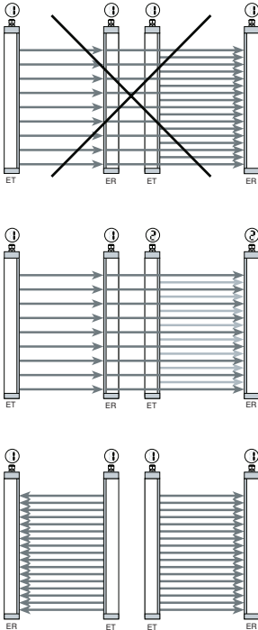
Fig. 7 Preventing mutual interference by selecting separate transmission channels
