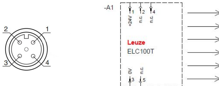
Fig. 6.1: Transmitter pin assignments and connection diagram
