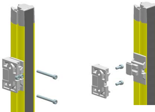
Fig. 5.8: Mounting via swiveling mounting brackets BT-2SB05 and M5 screws
