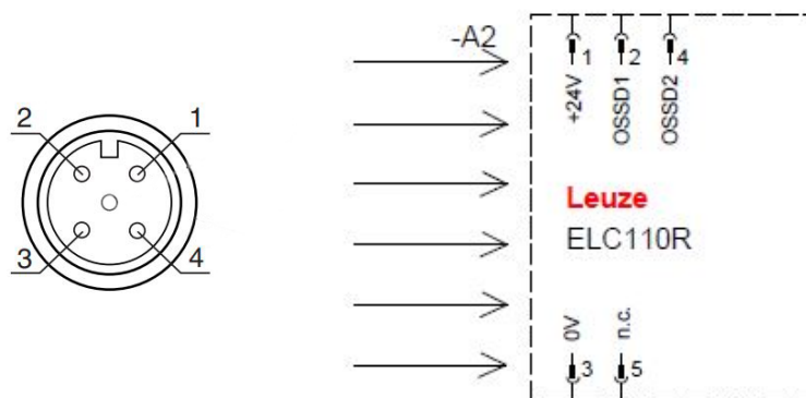
Fig. 6.2: Receiver pin assignment and connection diagram
