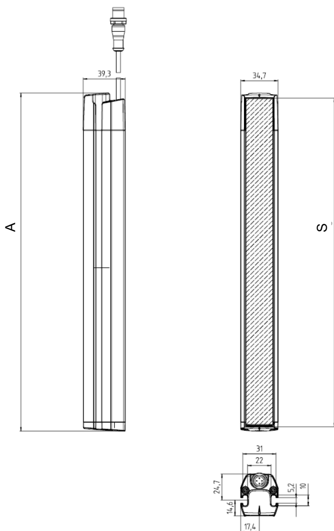
Fig. 12.1: Dimensions of transmitter and receiver
