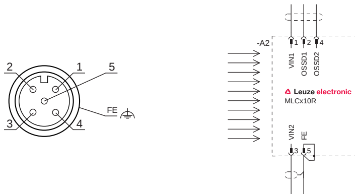
Fig. 7.3: Receiver pin assignment and connection diagram
