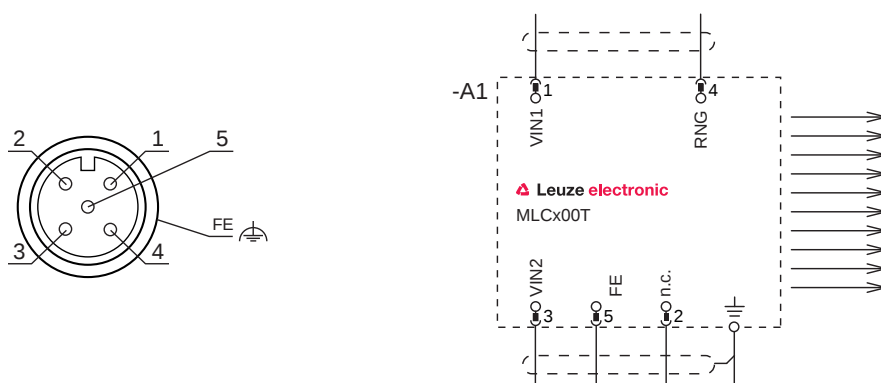
Fig. 7.1: Transmitter pin assignments and connection diagram
