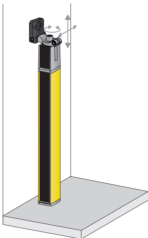
Fig. 6.10: Mounting directly on the machine table
