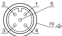
Fig. 7.1: Transmitter pin assignment
