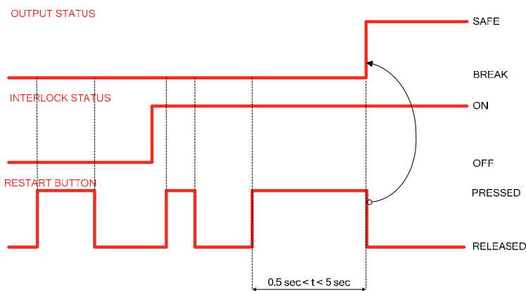
Fig. 8.6: Manual reset time
