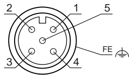
Fig. 7.2: Receiver pin assignment
