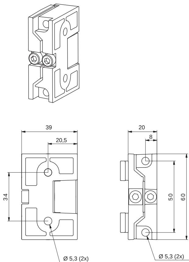
Figure 16.7 : Supports pivotants BT-2SB10/BT-2SB10-S
