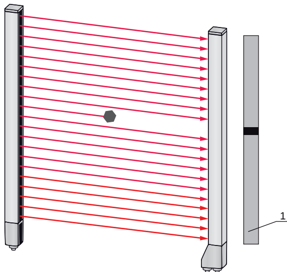
Figure 4.7 : Configuration de lissage "1"
