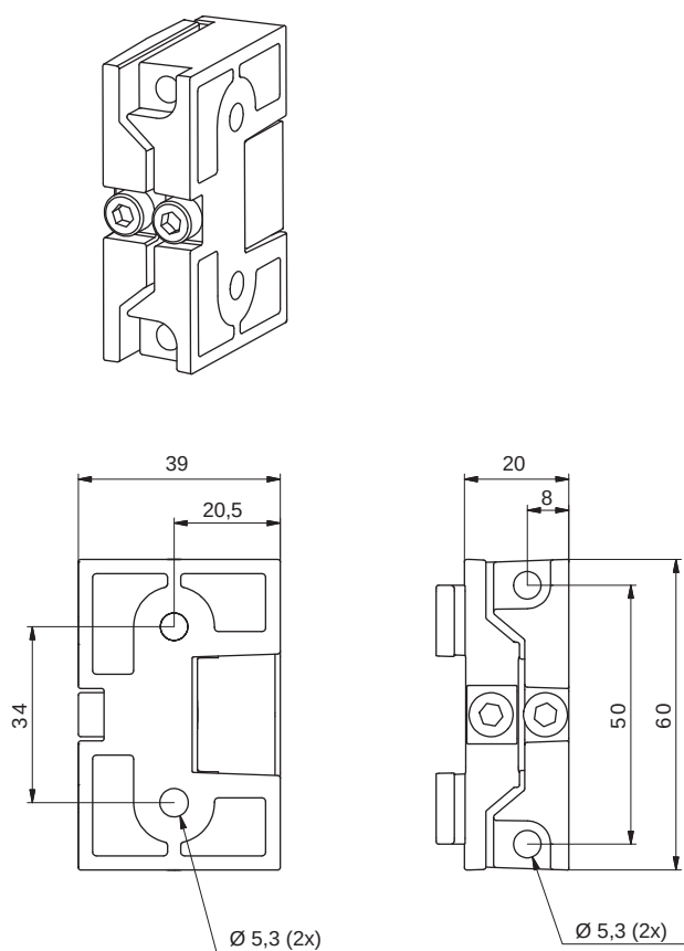
Figura 20.8: Supporti orientabili BT-2SB10/BT-2SB10-S
