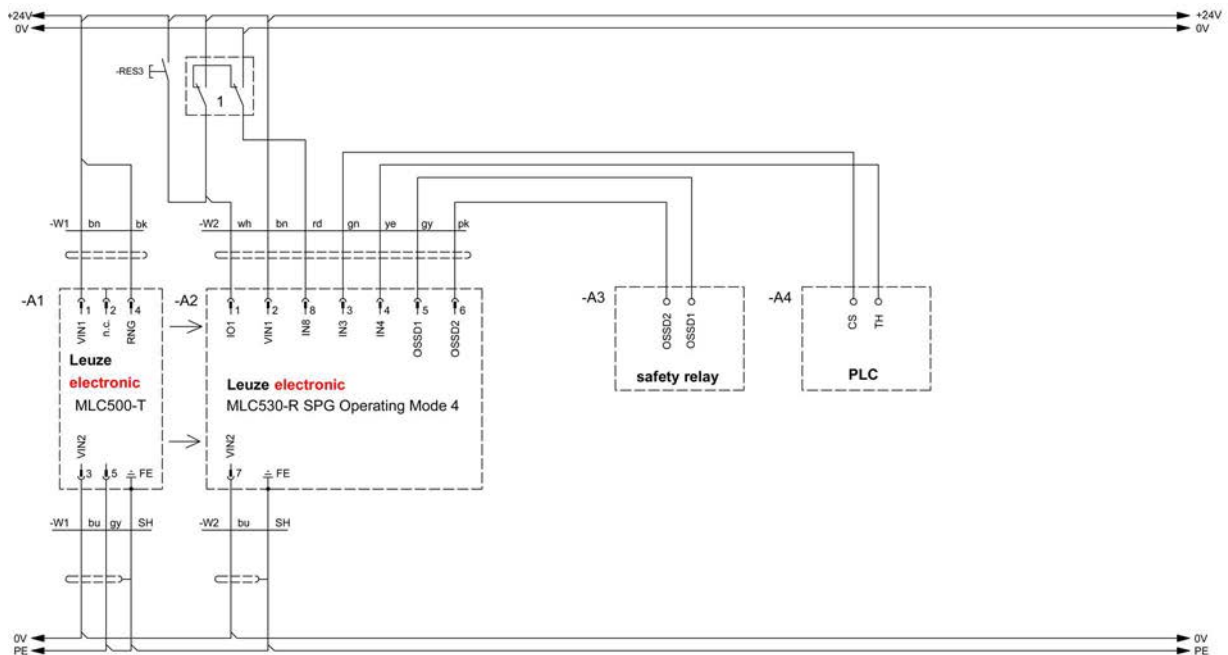
Fig. 8.5: Operating mode 4: circuit diagram example with Smart Process Gating (SPG)
