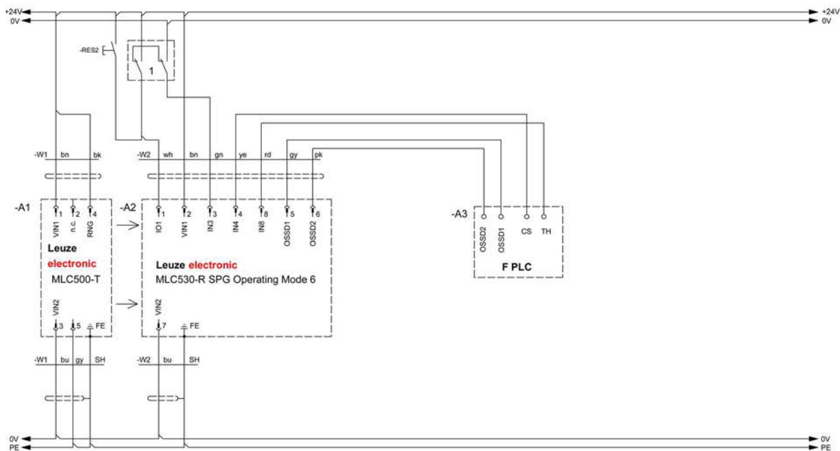
Fig. 8.7: Operating mode 6: circuit diagram example with Smart Process Gating (SPG)
