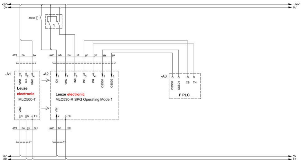
Fig. 8.4: Operating mode 1: connection example with Smart Process Gating (SPG)
