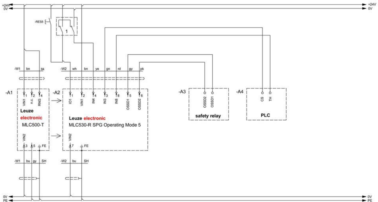
Fig. 8.6: Operating mode 5: circuit diagram example with Smart Process Gating (SPG)
