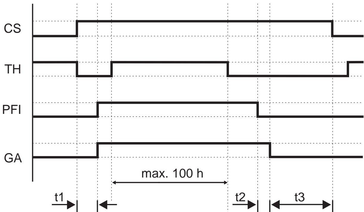
Fig. 4.9: Prolongation du time-out de SPG
