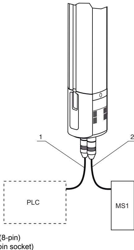
Figure 4.8: 2nd muting signal from the control
