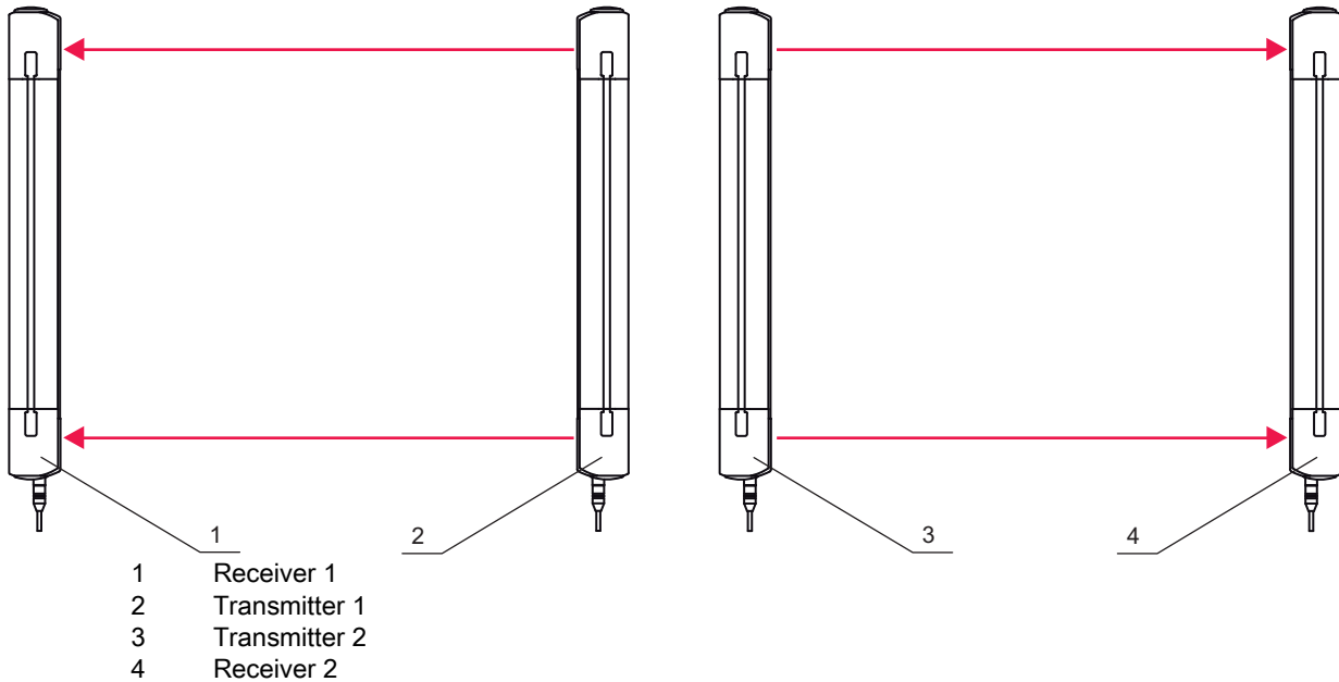
Figure 6.7: Opposing mounting
