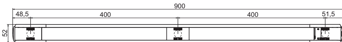
Figure 14.3: Dimensions of MLD, 3-beam transmitter, receiver
