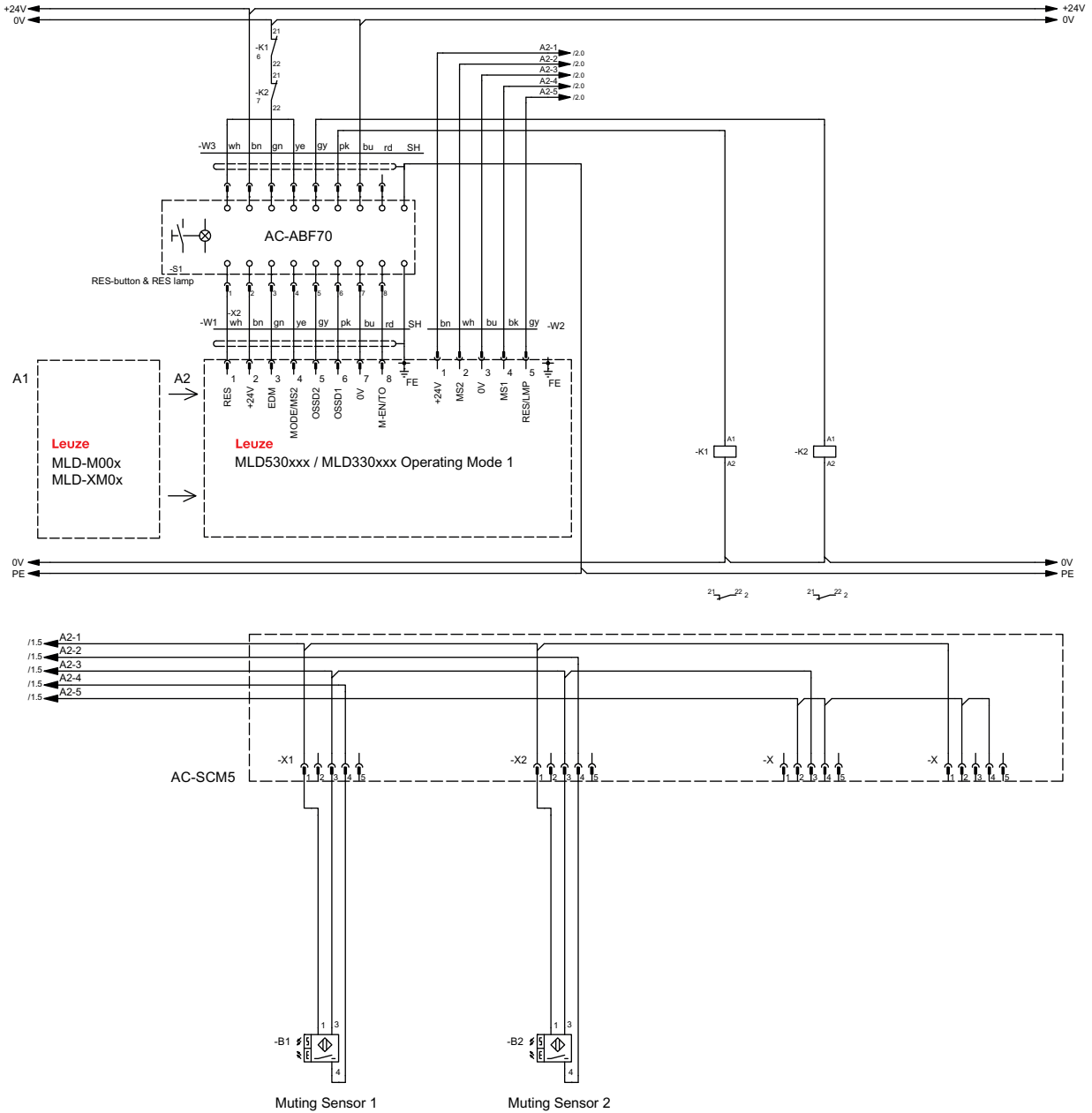
Figure 7.11: Connection example MLD 330, MLD 530 transceiver system: timing controlled 2-sensor muting with muting timeout 10 min
