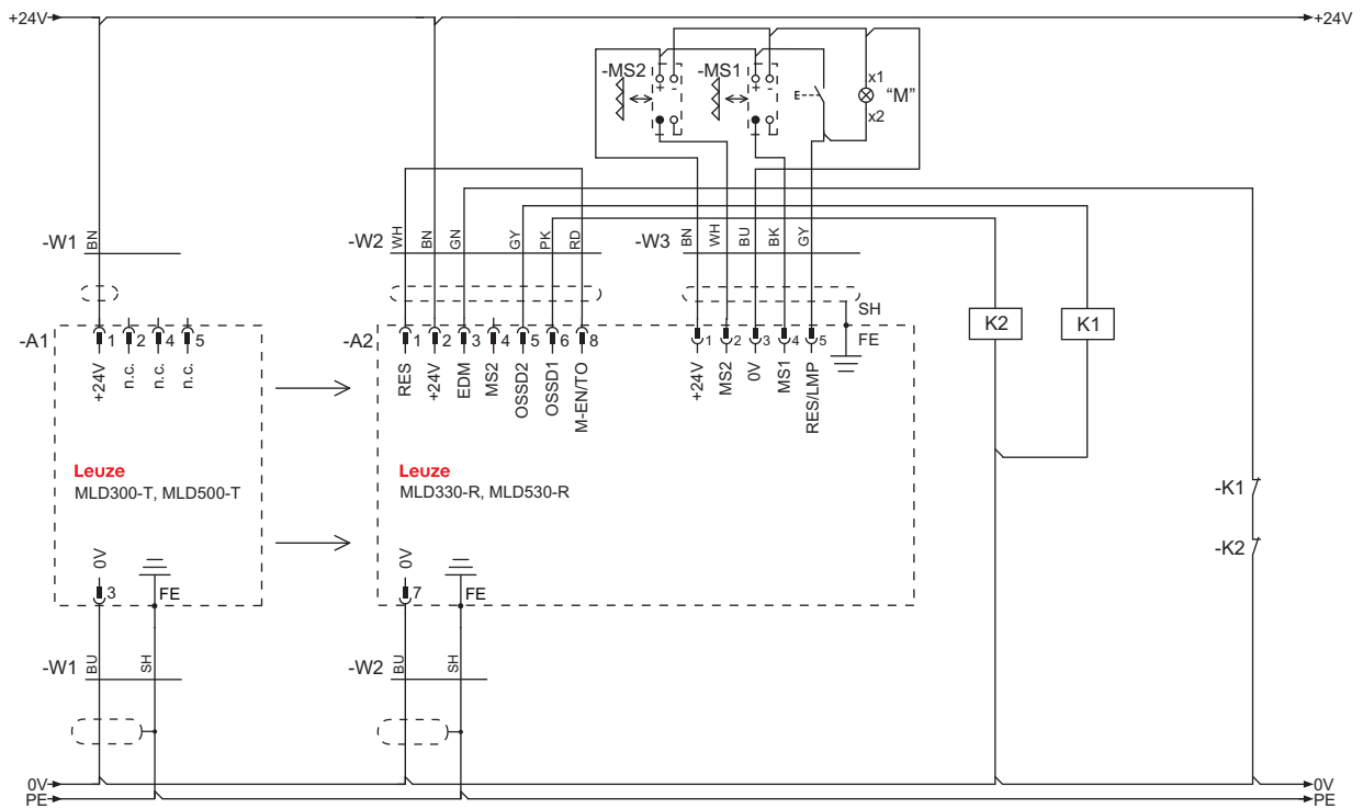
Figure 7.13: Connection example MLD 330, MLD 530 (transmitter-receiver system): timing controlled 2-sensor muting with muting timeout 100 h (transceiver connected in an analogous manner)
