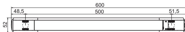
Figure 14.2: Dimensions of MLD, 2-beam transmitter, receiver
