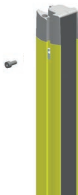
Fig. 5.6: Mounting via sliding blocks
