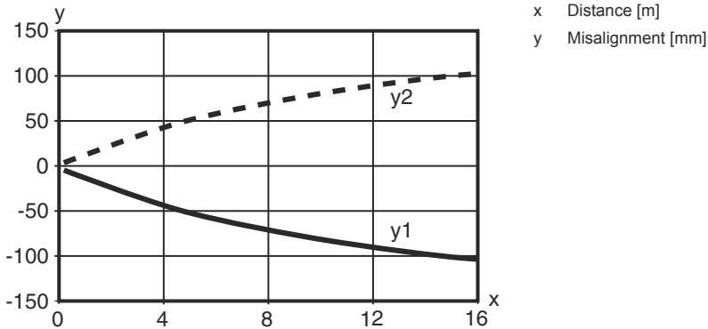
Typ. response behavior (TKS100x100)
