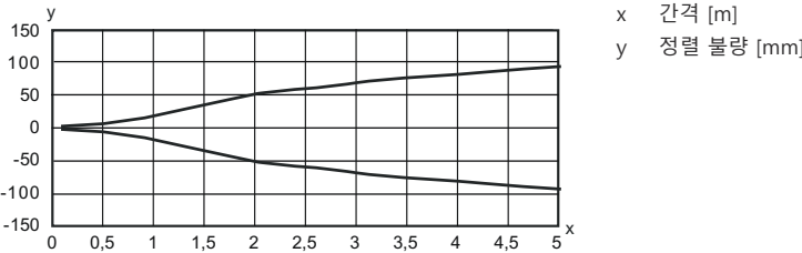
전형적인 반응 거동(TKS100x100)
