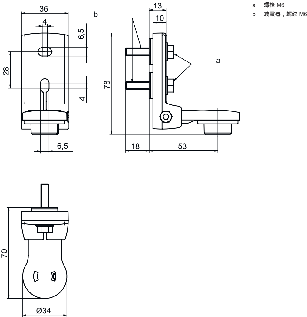
旋转架 BT-SET-240BS-E
