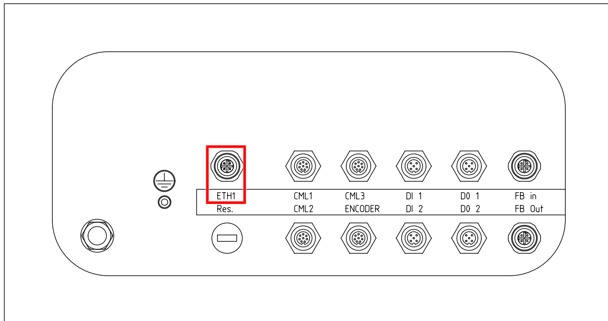
Fig. 6.6: Connexion Ethernet TCP/IP
