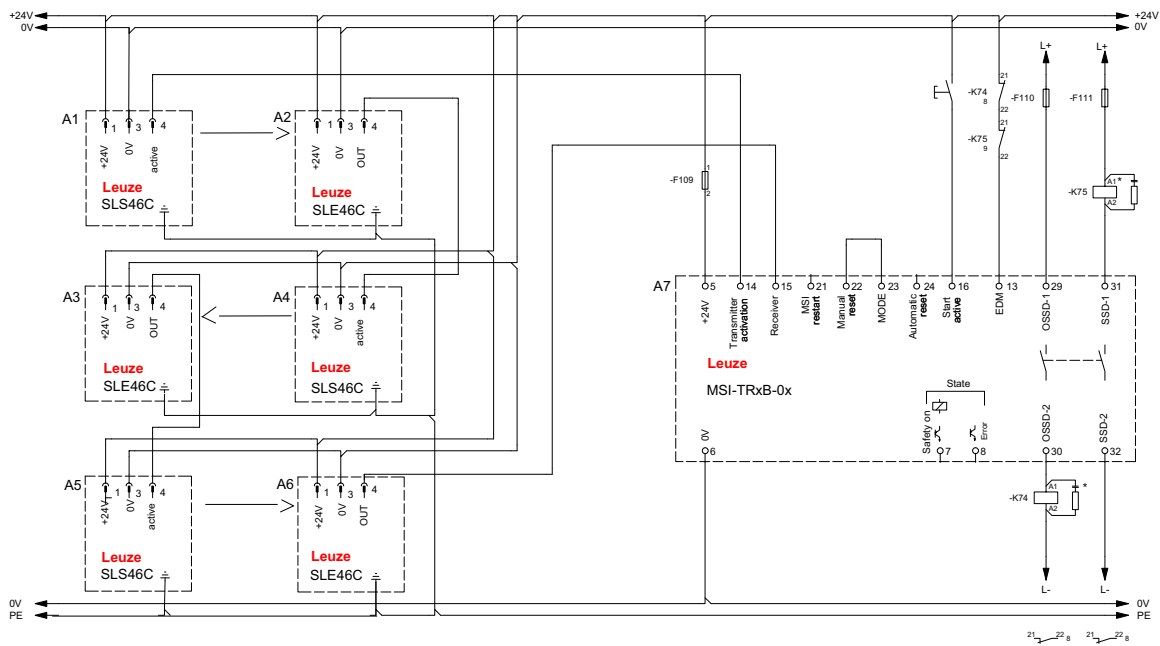
Figure 7.3: MSI-TRxB-xx safety relay with 3x SLS 46C type 2 single light beam safety devices in series, start/restart interlock (RES) and external contactor monitoring (EDM).
