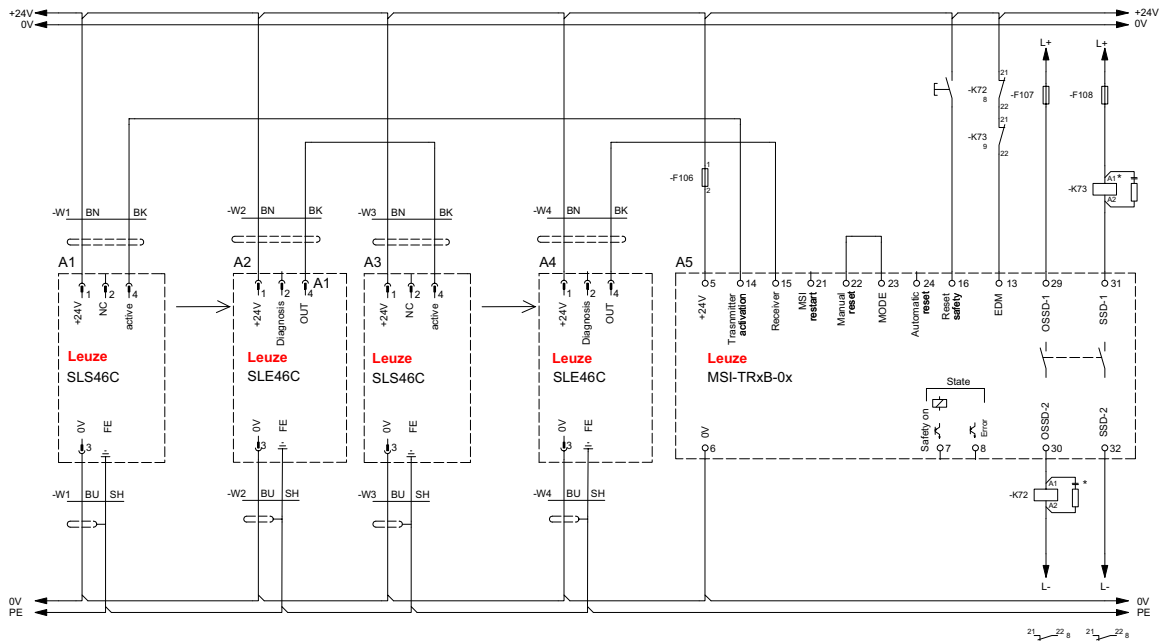
Figure 7.2: MSI-TRxB-xx safety relay with 2x SLS 46C type 2 single light beam safety devices in series, start/restart interlock (RES) and external contactor monitoring (EDM).
