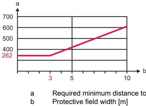
Figure 6.4: Minimum distance to reflective surfaces as a function of the protective field width up to 10 m
