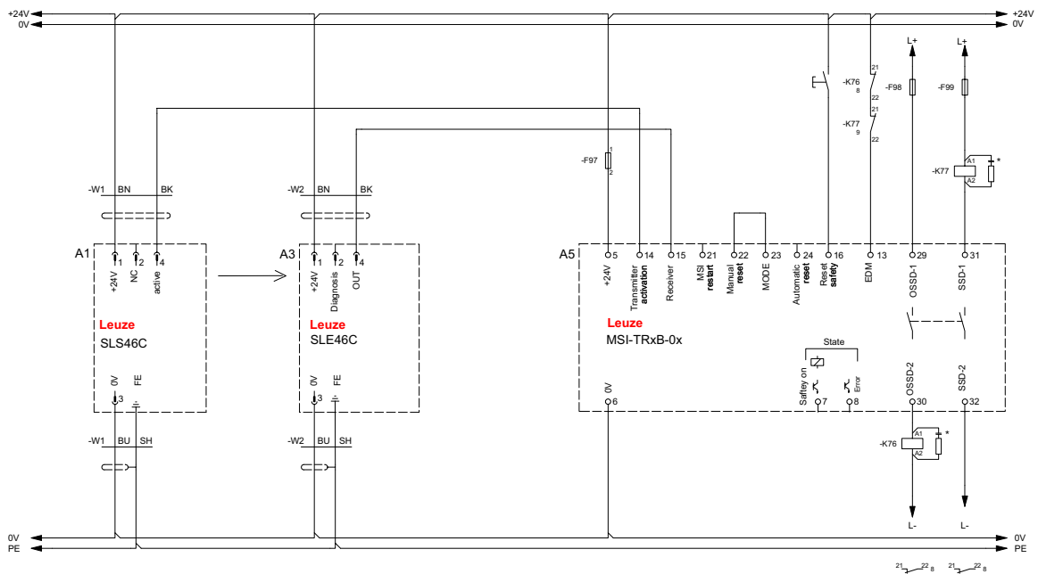
Figure 7.1: MSI-TRxB-xx safety relay with type 2 SLS 46C single light beam safety device, start/restart interlock (RES) and external contactor monitoring (EDM).
