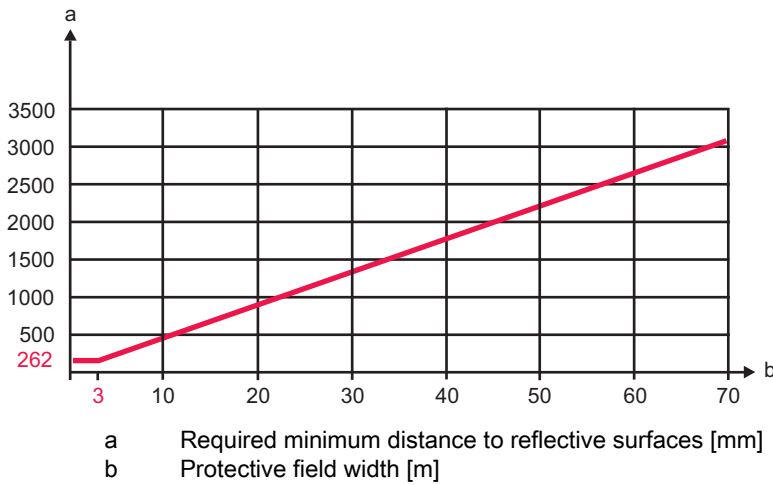
Figure 6.5: Minimum distance to reflective surfaces as a function of the protective field width up to 70 m
