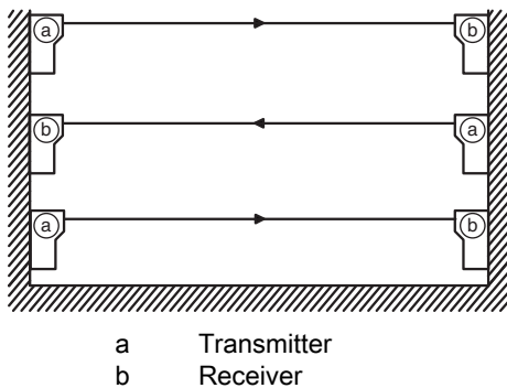
Figure 6.2: Multi-axis arrangement
