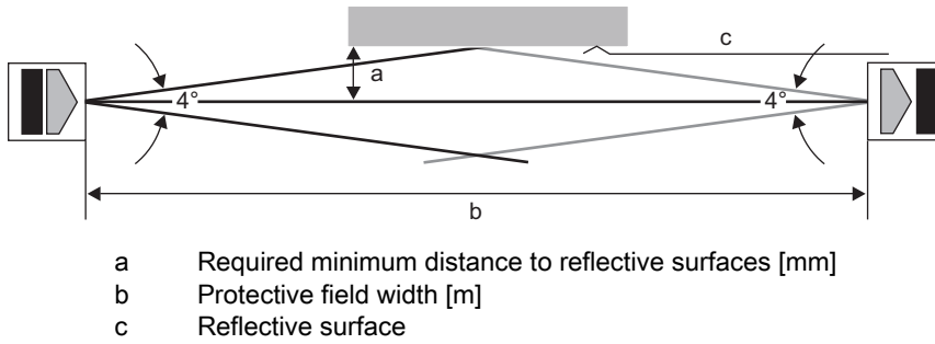
Figure 6.3: Minimum distance to reflective surfaces depending on protective field width
