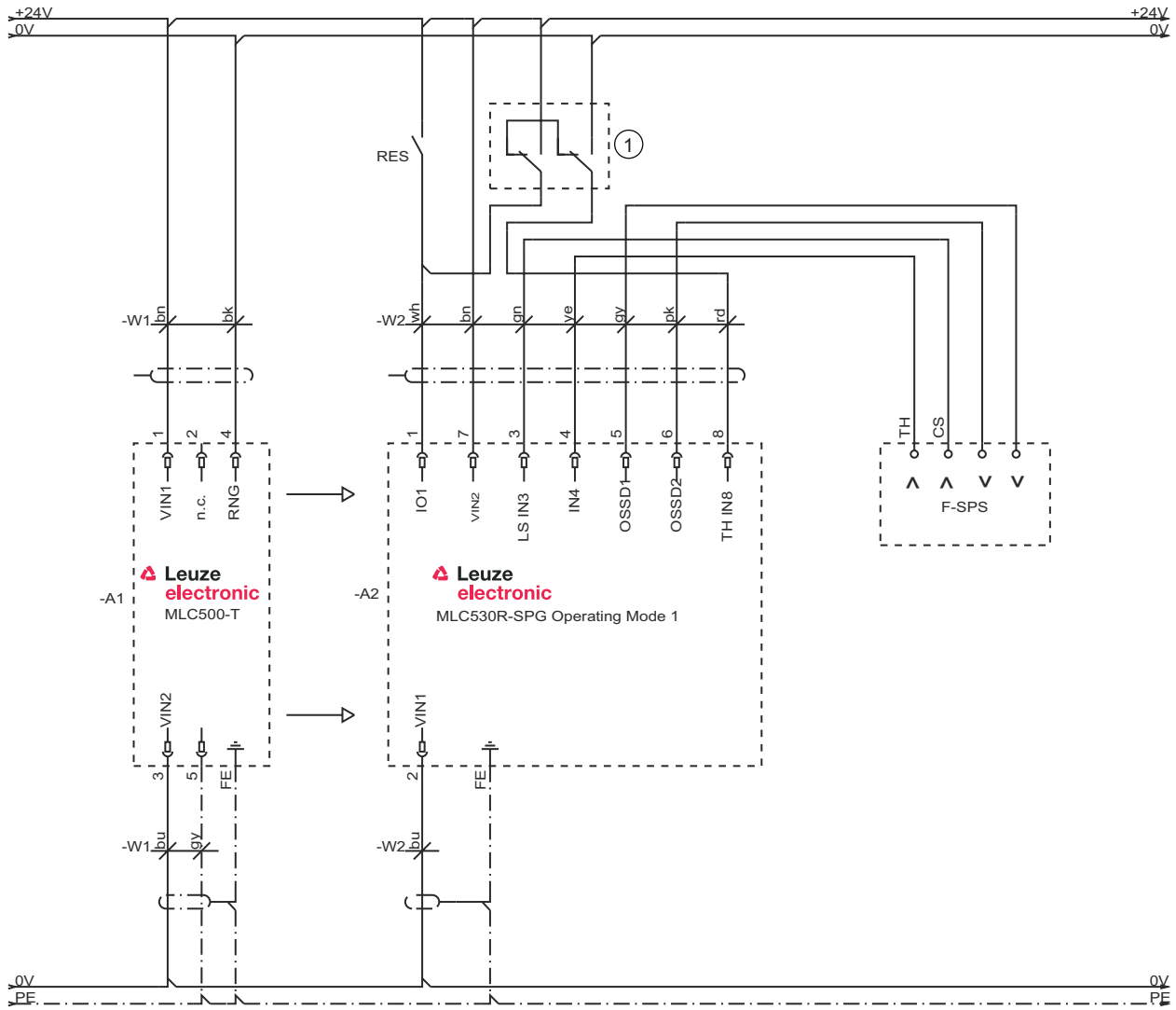
1 Optionaler Einlern-Schlüsseltaster
