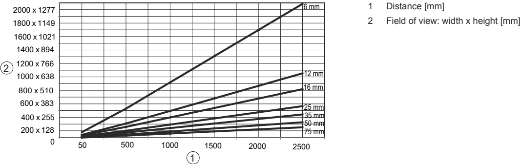
Relationship between working distance and field of view size
