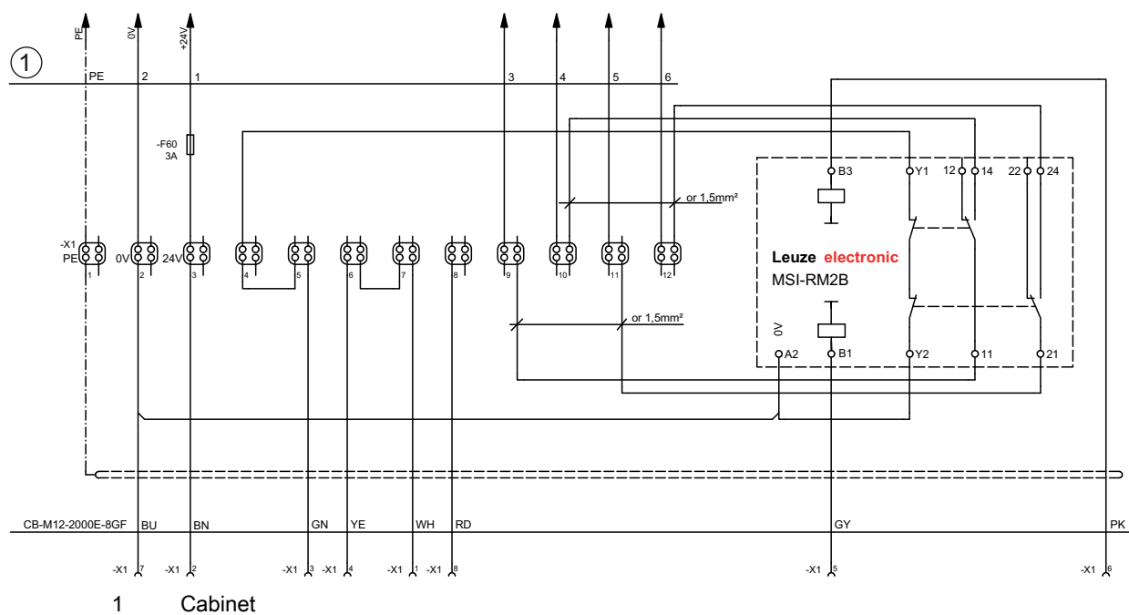
Figure 6.1: Circuit plan – ML2R-RM2
