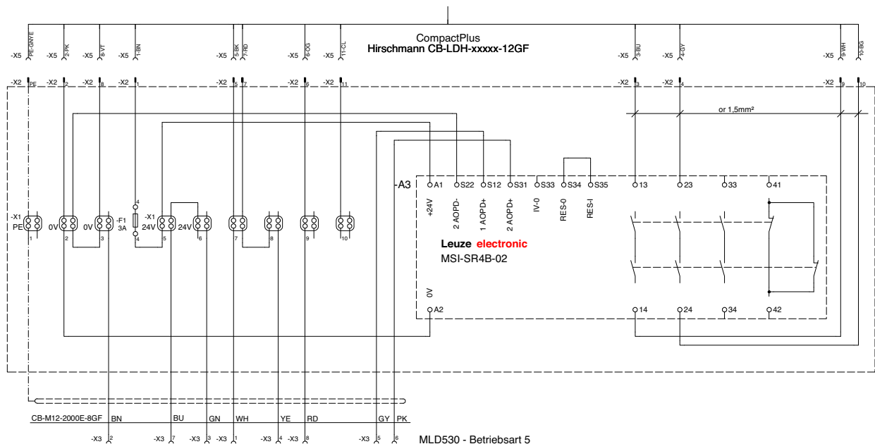
Figure 6.1: Circuit plan – ML2R-SR4
