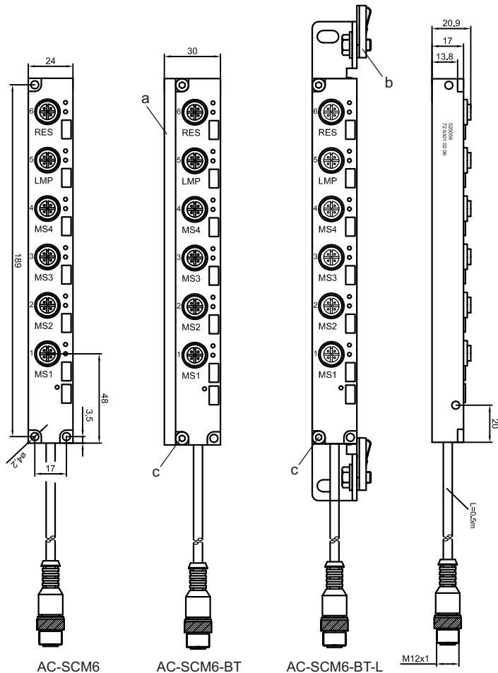
a = Montageplatte b = Nutenstein c = Zylinderschraube M4x22
